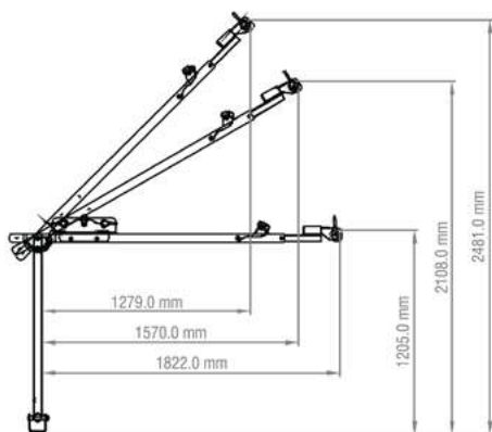
Minimum Extension Positions
