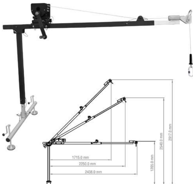
Full Extension Positions
